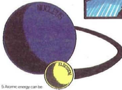
4 Within the atom, each electron spins around the nucleus in much the same way that the earth revolves around the sun. (Remember how the earth revolves around the sun? If you've forgotten, turn back to Unit 8. Our Solar System.)
